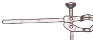
LS - CCL.6 CONDENSOR CLAMP, 3 finger type , jaws of Brass casting, operated by a key, fitted with 300 mm long M.S. Rod Suitable to hold upto 75 mm dia rod.
