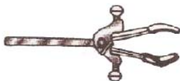
LS- CCL.7 CONDENSOR CLAMP (Fisher type) 3 finger type of jaws of Aluminium, operated by double key, to hold objects upto 100 mm dia rod, fitted with 300 mm long M.S.Rod.
